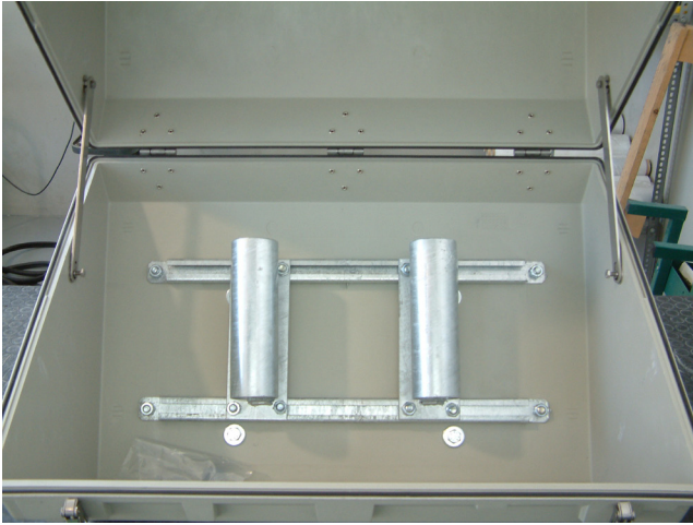
enclosure model 700 fitted with bracket model SP-I2
