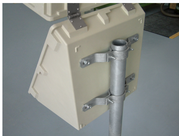
enclosure model 500 fitted with bracket model SP-S2
