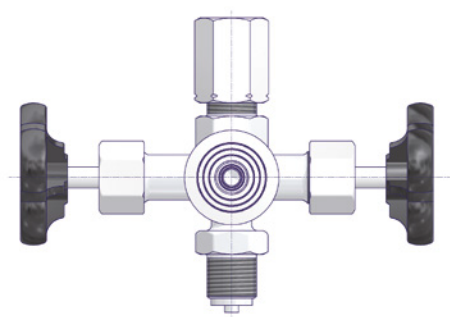
Valve with Test Flange Ø 40 x 5
