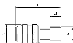
Male Thread
