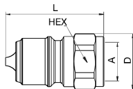
Female Thread
