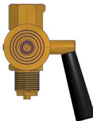
Gauge Cock with Test Flange Ø 40 x 5
