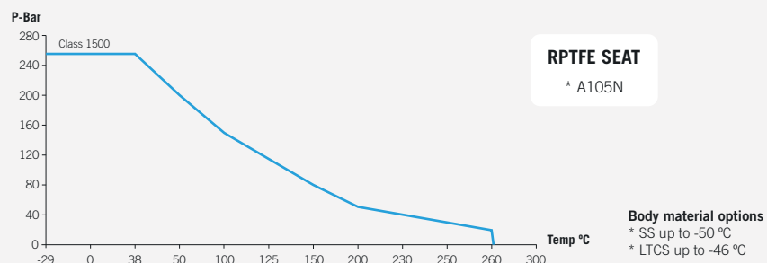
Fig. 41500 (Class 1500)
