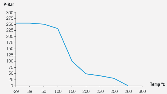
PEEK (Class 2500)
