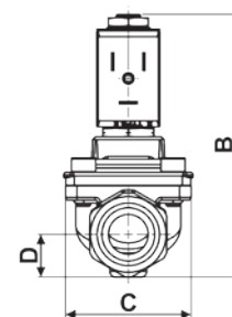
Flow direction overseat 1 → 2
