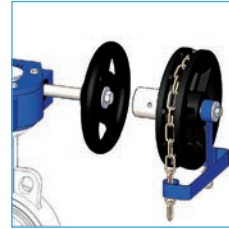
KCAT Kit comando a catena (4 m) Chain driver (4 m) (Jg DN 25-400 Lg DN 25-300)
