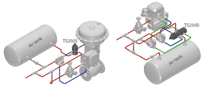
<Single Acting Linear Actuator>
