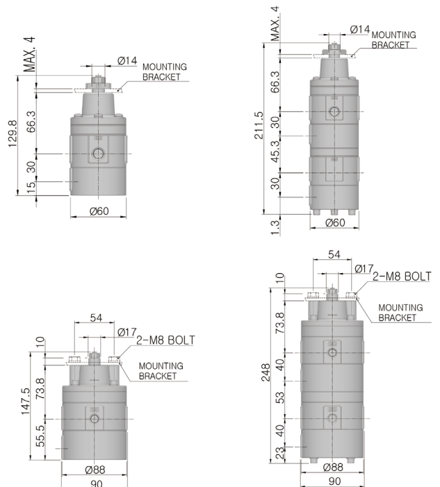
<Single Acting Linear Actuator>
