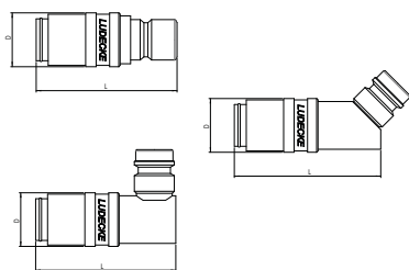
adaptery systemowe ESHM
