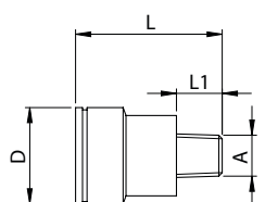
gniazdo z gwintem zew.
