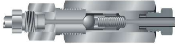
Ball Type Check Valve
