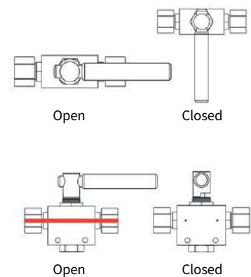
2-Way open & close position
