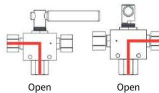
3-Way open &amp; close position – 90° Diverter
